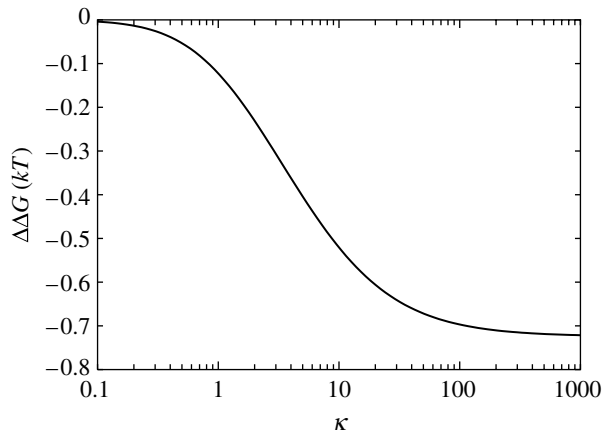
Figure 9. Allosteric free energy \Delta\Delta G against clamping \kappa = k_1/k_0 = k_{-1}/k_0 showing the effect of clamping on the allosteric free energy for coiled geometry for slide and bend fluctuations.
